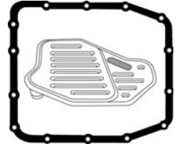
14 Bolt Pan AOD-E (92-95) 2WD 4R70W (93-95) 2WD FK53423D
